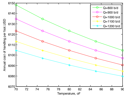
Figure 3: Temp against cost of handling ( f_o = 0.7 )
