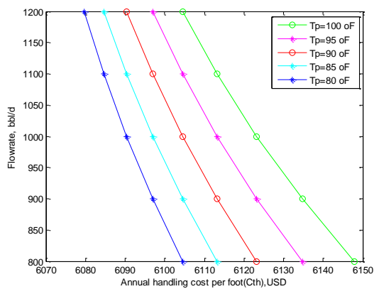
Fig 13: Cost of handling against flowrate ( f_o=0.7 )
