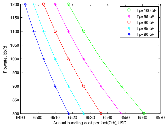
Fig 11: Cost of handling against flowrate ( f_o=0.8 )
