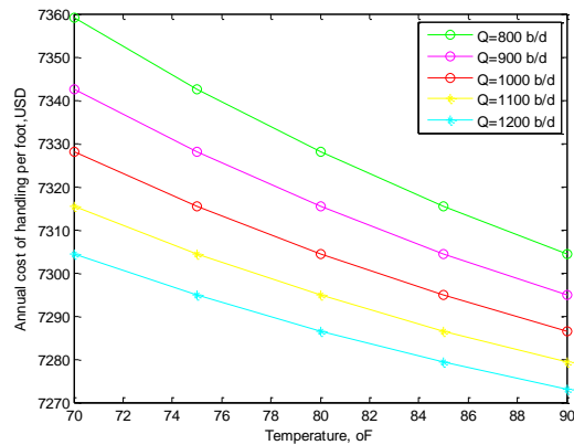
Figure 4: Temp against cost of handling ( Ca = 0.3 )
