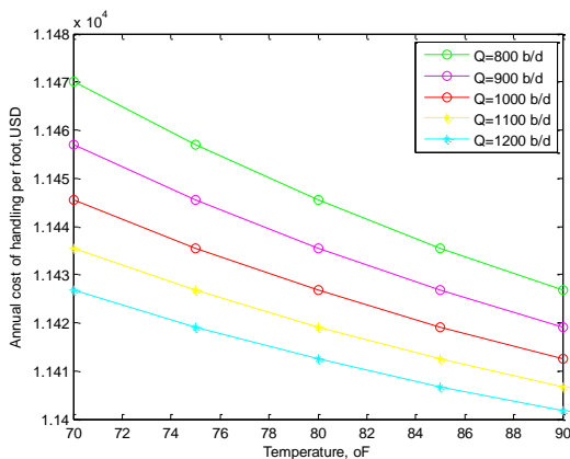
Figure 8: Temp against cost of handling ( P = 25 )
