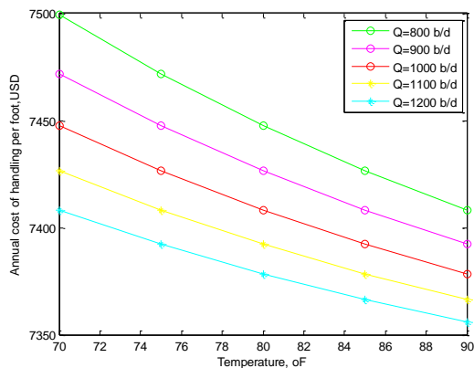
Figure 5: Temp against cost of handling ( Ca = 0.5 )
