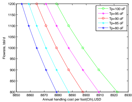
Fig17: cost of handling against flowrate ( P = 15 )
