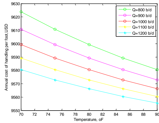
Fig 9: Temp against cost of handling ( C_{cPB} = 700 )
