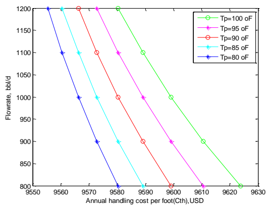
Fig 19: Temp against cost of handling ( C_{cPB} = 700 )
